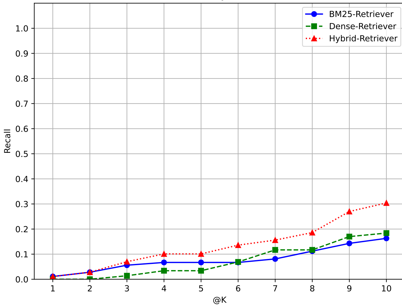
Query 23
